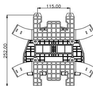
With Cable-storage-bracket
