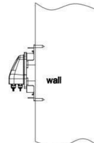
With Cable-storage-bracket
