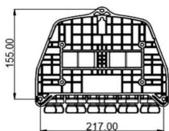
Without Cable-storage-bracket
