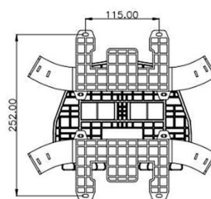
With Cable-storage-bracket
